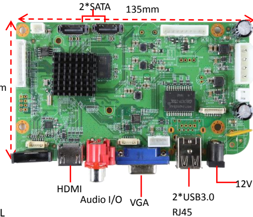
Model: NBD8025R-PL
